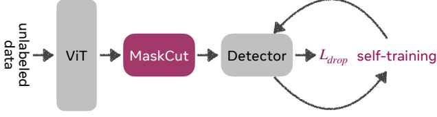
Figure 2. Overview of CutLER. We propose a simple yet effective method to train an object detection and instance segmentation model without using any supervision. We first propose MaskCut to extract initial coarse masks from the features of a self-supervised ViT. We then learn a detector using our loss dropping strategy that is robust to objects missed by MaskCut. We further improve the model using multiple rounds of self-training.
